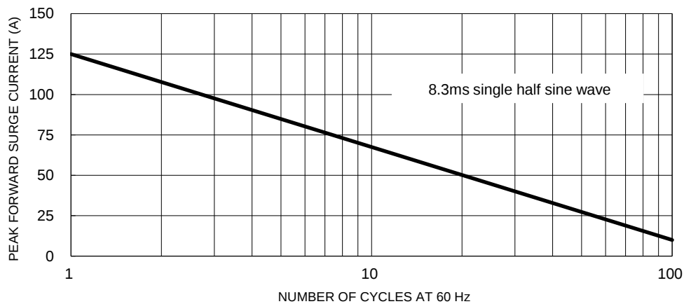
Fig.5 Maximum Non-Repetitive Forward Surge Current
